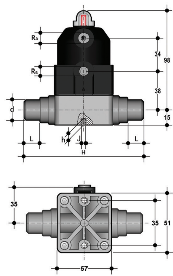
CMDM/CP NO Compact diaphragm valve with male ends for pneumatically actuated socket welding, Normally Open function
