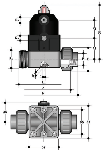
CMUFV/CP NC Compact diaphragm valve with female union ends, pneumatically actuated gas cylinder thread, Normally Closed function
