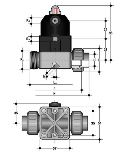
CMUIF/CP NO Compact diaphragm valve with female union ends for pneumatically actuated socket welding, Normally Open function
