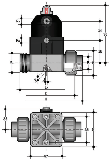
CMUFV/CP NO Compact diaphragm valve with female union ends, pneumatically actuated gas cylinder thread, Normally Open function
