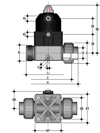
CMUIF/CP DA Compact diaphragm valve with female union ends for pneumatically actuated socket welding, Double-Acting function
