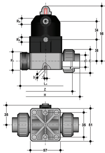
CMUIV/CP NC Compact diaphragm valve with female union ends for solvent welding, pneumatically actuated metric series, Normally Closed function
