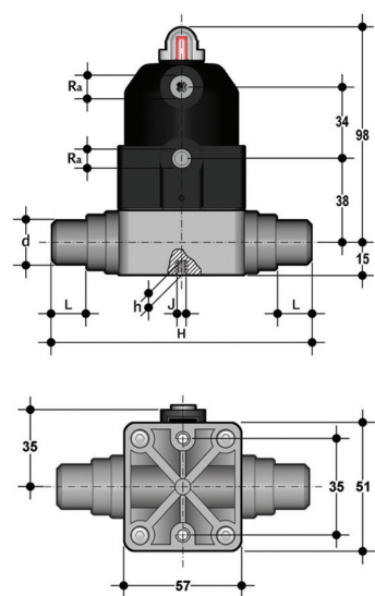
CMDF/CP NO Compact diaphragm valve with male ends for pneumatically actuated socket welding, Normally Open function
