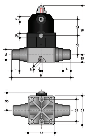
CMDM/CP NC Compact diaphragm valve with male ends for pneumatically actuated socket welding, Normally Closed function
