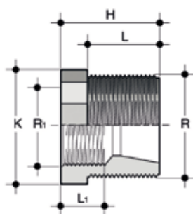
Fig. B RFV Reducer with BSP threaded male end (R) and BSP threaded female end (R1 reduced) (fig. B)
