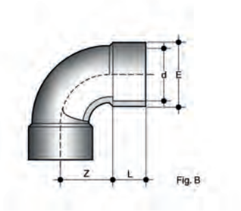
GIC 90° elbow with solvent weld sockets (fig. B)
